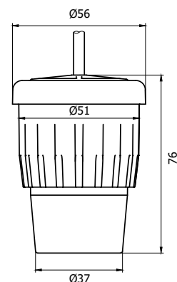
Dimensions mm
